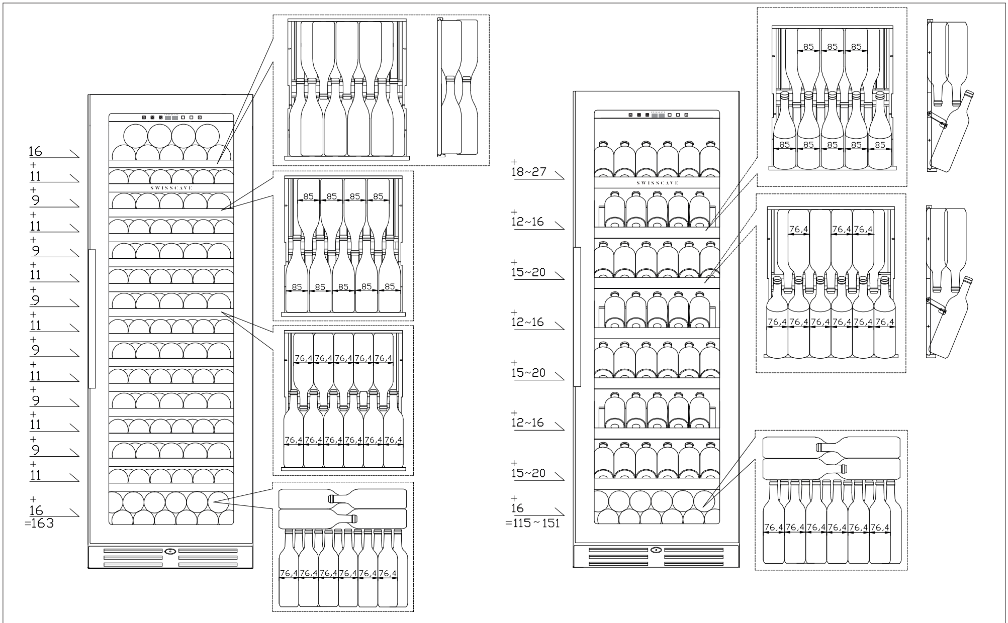
Loading view drawing for WLB-460FL-MIX (left) and WLB-460FLD-MIX (right)
